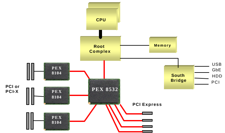
Figure 1. Fan-in/out Usage
