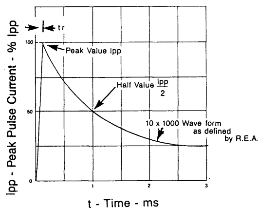
Test waveform parameters: t_r = 10 \mu s , t_p = 1000 \mu s FIGURE 2 Pulse Waveform
