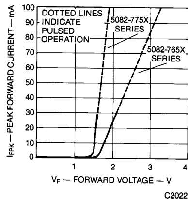
Fig. 6. Peak Forward Current vs. Forward Voltage
