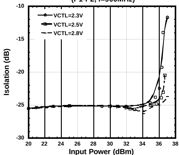
Isolation vs. Input Power
