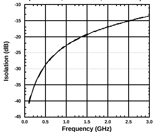
P1-P4 Isolation vs.Frequency (VCTL1=0V, VCTL2=2.8V, Pin=-10dBm)
