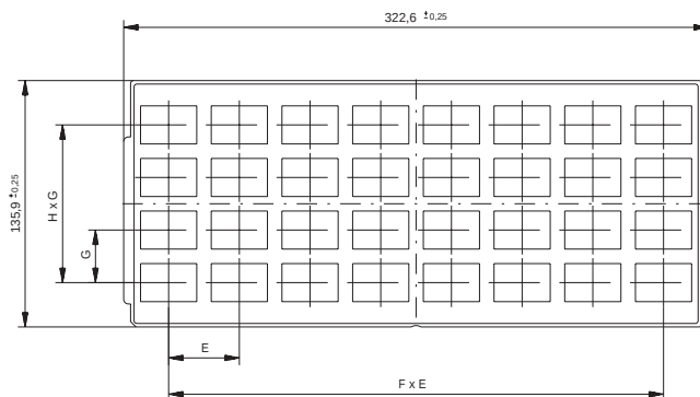
Tray packaging (9pin version pictured)
