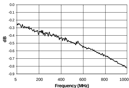
Amplitude Unbalance
