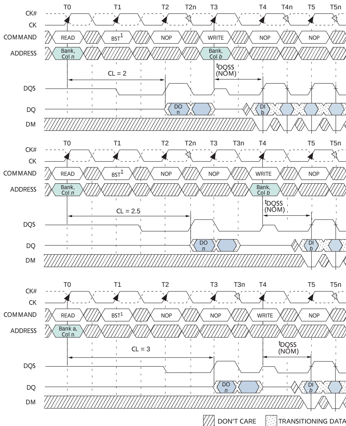
Figure 30: READ-to-WRITE
