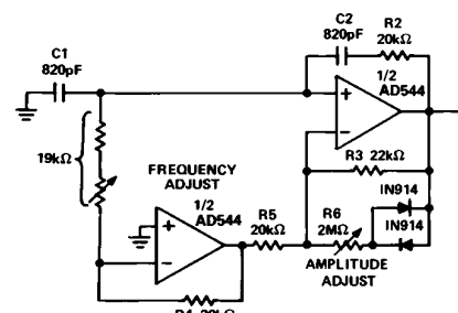
Figure 36. Wien-Bridge Oscillator- f_0 = 10 kHz
