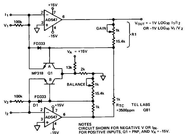
Figure 33. Log-Ratio Amplifier
