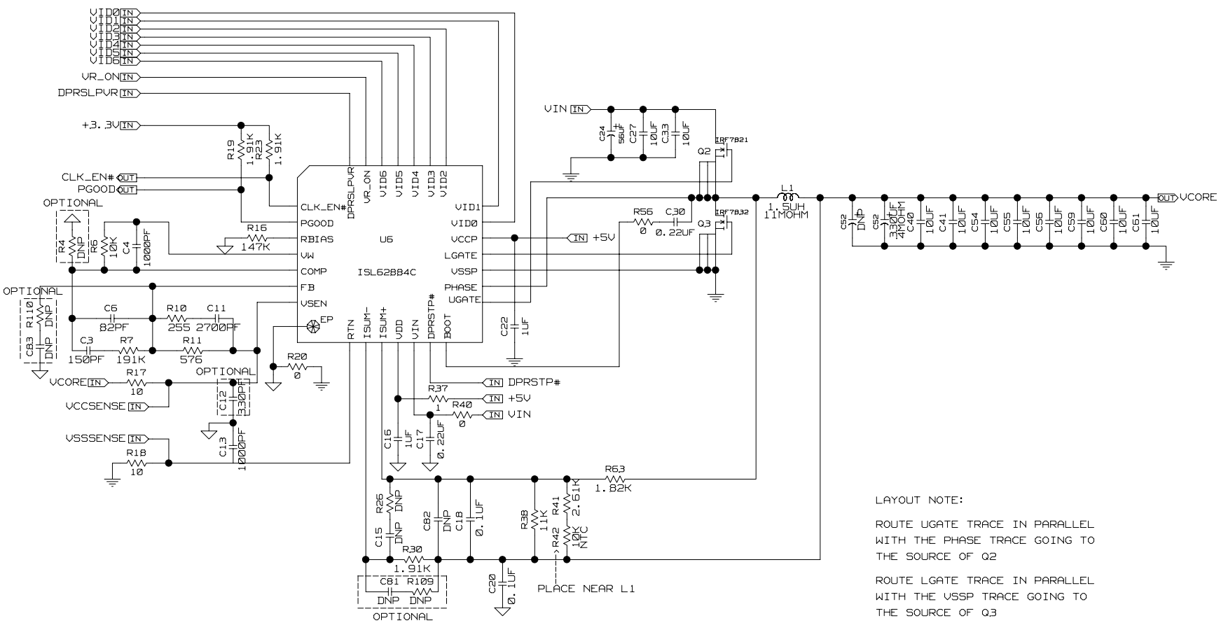
FIGURE 22. REFERENCE DESIGN
