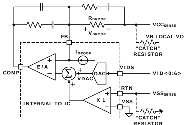
FIGURE 9. DIFFERENTIAL SENSING AND LOAD LINE IMPLEMENTATION
