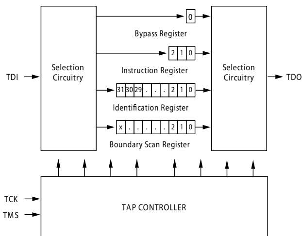
Figure 3. TAP Controller Block Diagram
