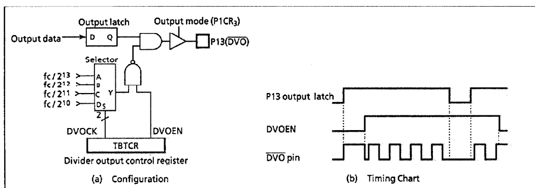
Figure 2-9. Divider output
