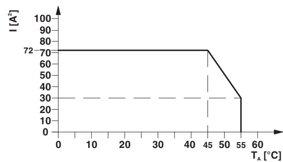
Figure 2 Derating curve
