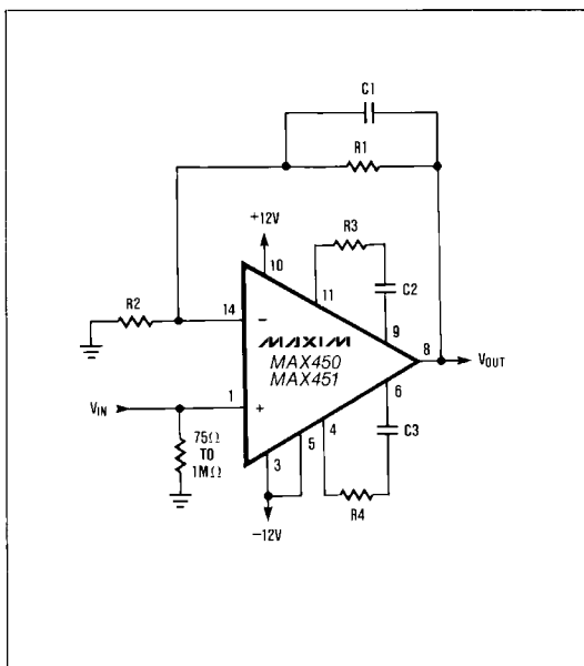
Figure 1. Non-inverting Configuration.
