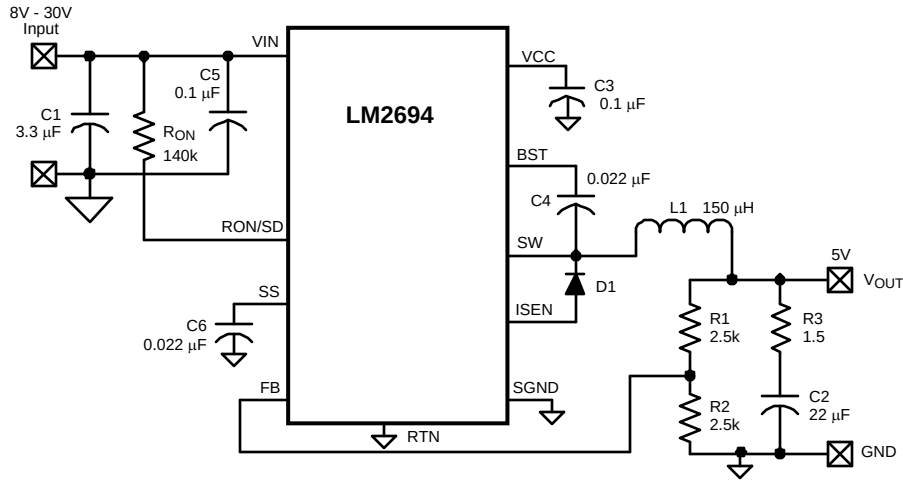
Figure 14. Example Circuit
