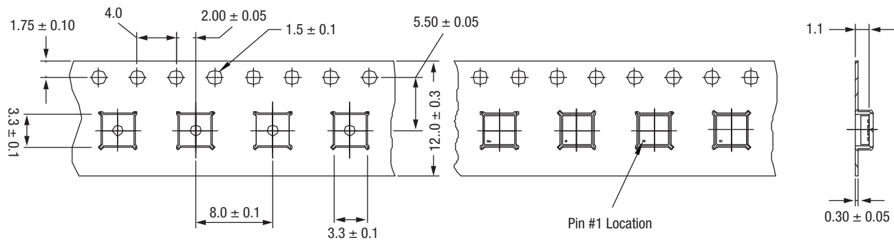
Figure 27. AAT1153 Tape and Reel Dimensions
