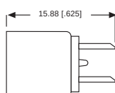
CONNECTOR 515-0012
