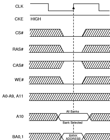
Figure 20 PRECHARGE COMMAND
