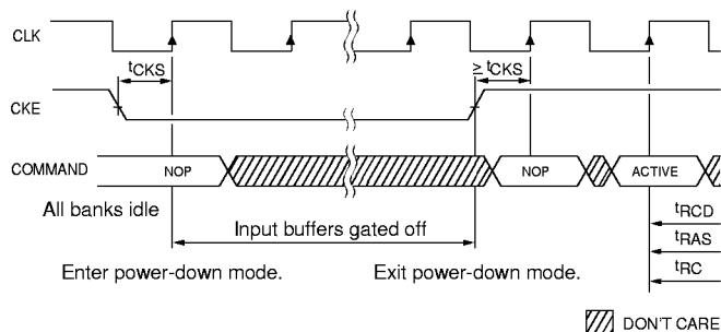
Figure 21 POWER-DOWN
