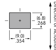
Maximum Panel Thickness .197" (5.0mm)
