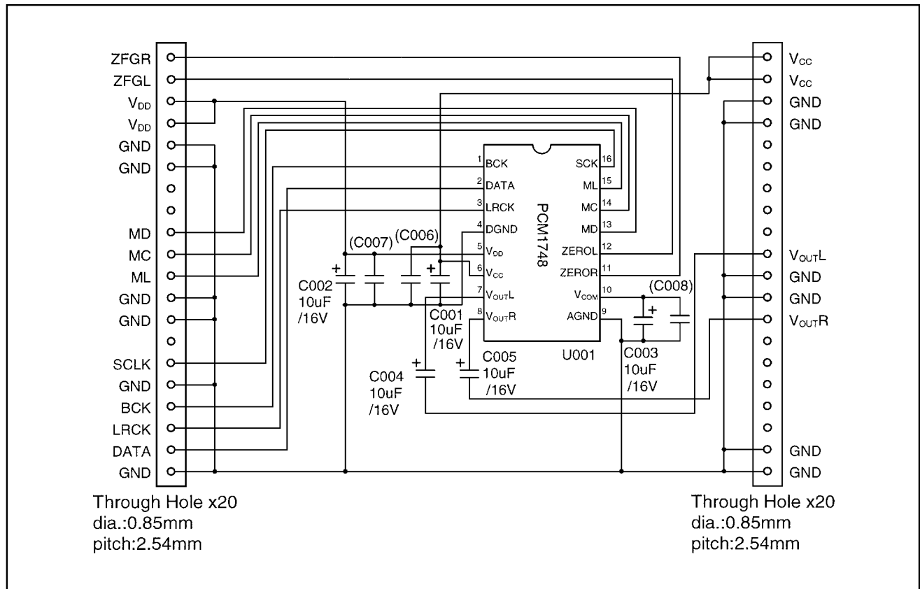
FIGURE 4. PCM1748 Daughter Card Schematic.
