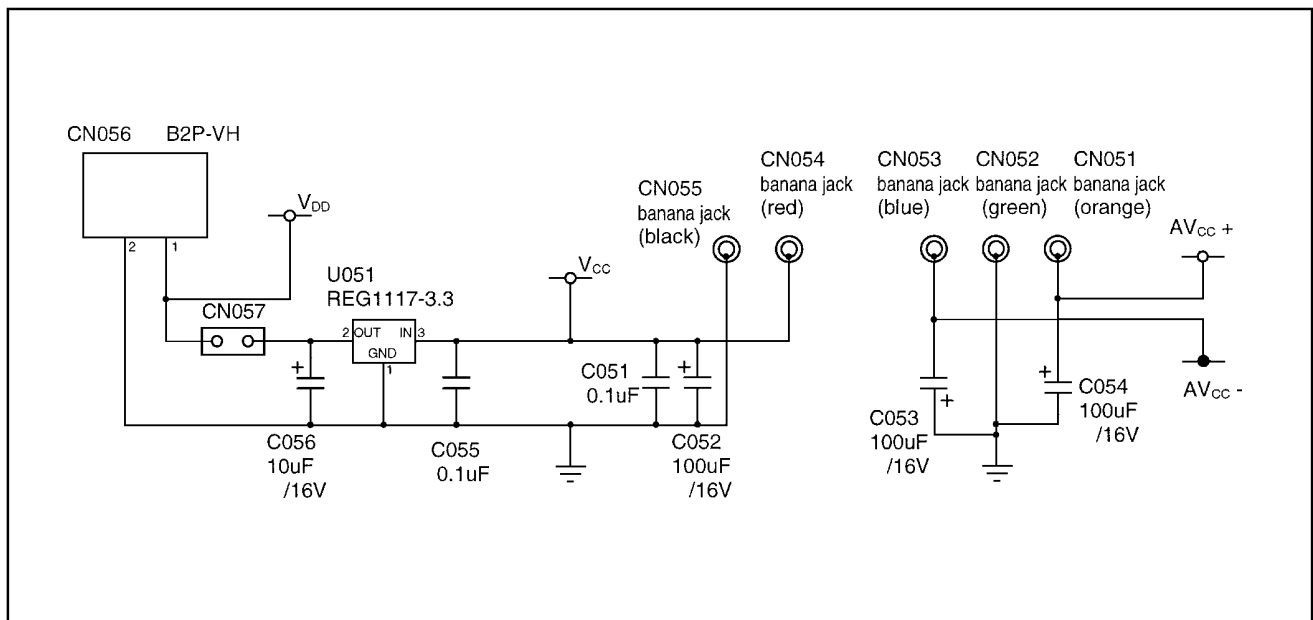
FIGURE 2. Power-Supply Connections.
