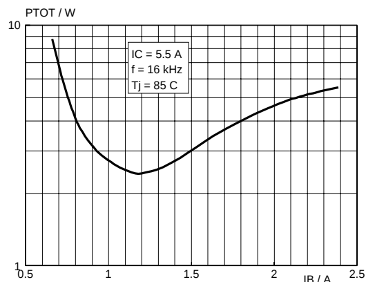
Fig.11. Limit P_{tot} ; T_J = 85^\circ\text{C} P_{tot} = f(I_{B(end)}) ; I_C = 5.5\text{ A} ; f = 16\text{ kHz}
