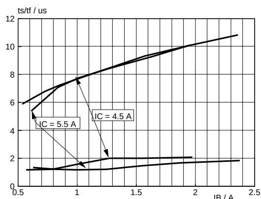
Fig.12. Limit storage and fall time. t_s = f(I_B) ; t_f = f(I_B) ; Parameter I_C ; T_J = 85^\circ\text{C} ; f = 16\text{ kHz}
