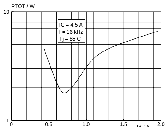
Fig.10. Limit P_{tot} ; T_J = 85^\circ\text{C} P_{tot} = f(I_{B(end)}) ; I_C = 4.5\text{ A} ; f = 16\text{ kHz}
