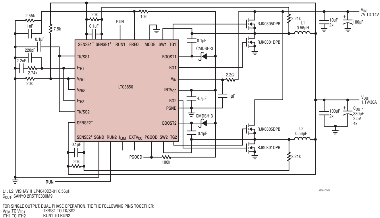
Figure 21. 1.1V/30A Dual Phase Core Converter, F_{SW} = 400kHz
