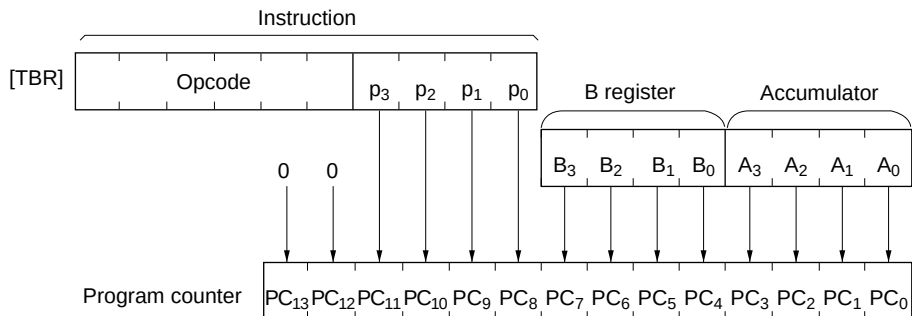
Figure 3-3 ROM Addressing Modes
