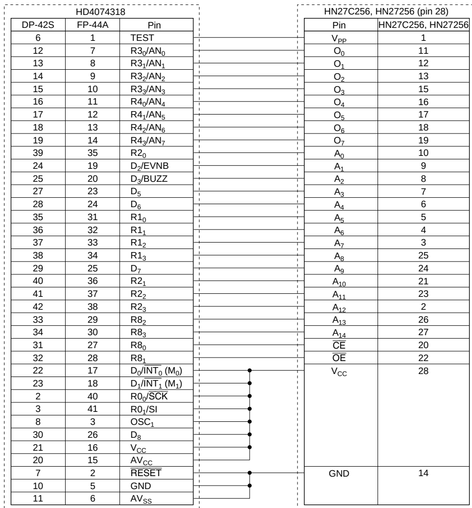
Figure 22-2 shows the HD4074318 socket adapter pin correspondence.
