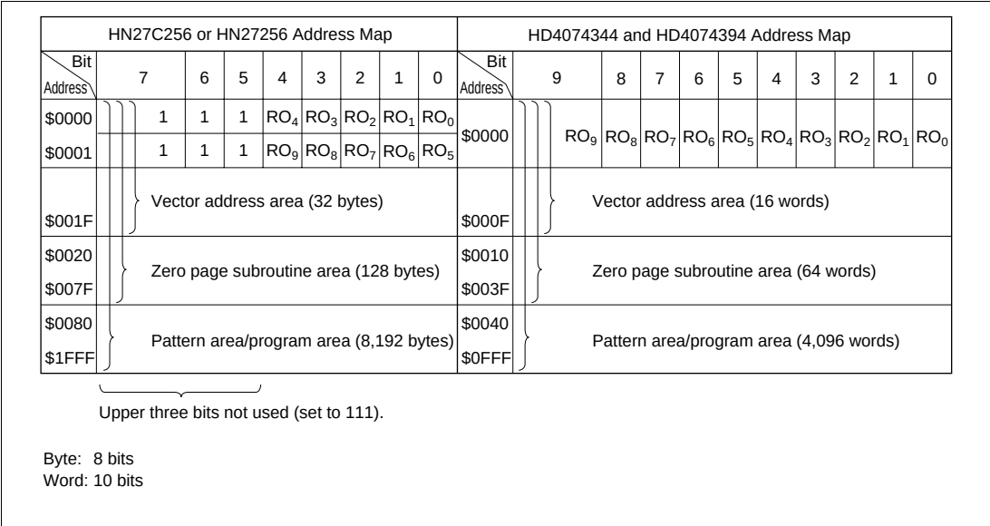
Figure 22-6 HD4074344 and HD4074394 PROM Mode Memory Map
