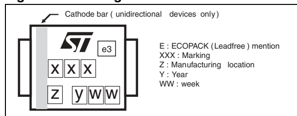
Figure 14: Marking
