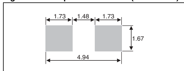
Figure 13: Foot print dimensions (millimeters)
