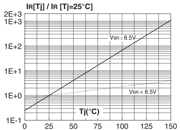
Figure 10: Relative variation of leakage current versus junction temperature
