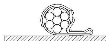
UGCTE Bundle is offset from mounting point
