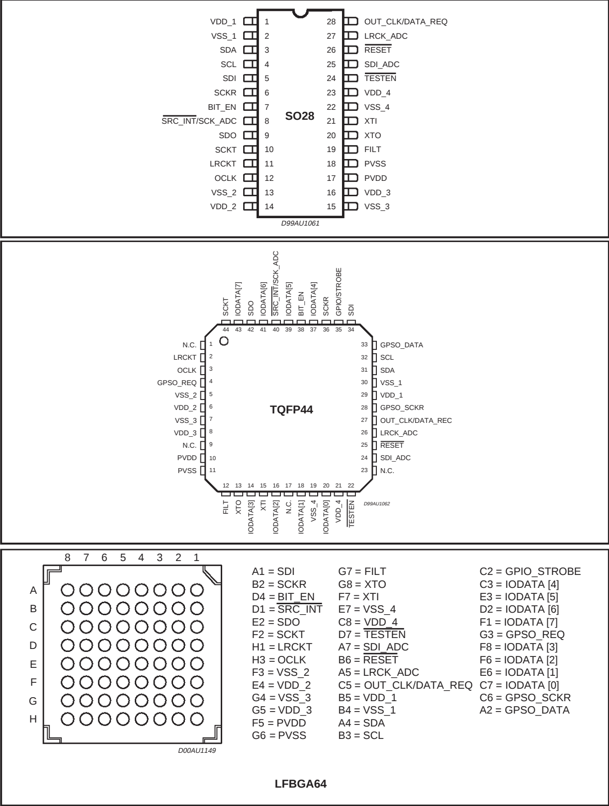
Figure 2. PIN CONNECTIONS
