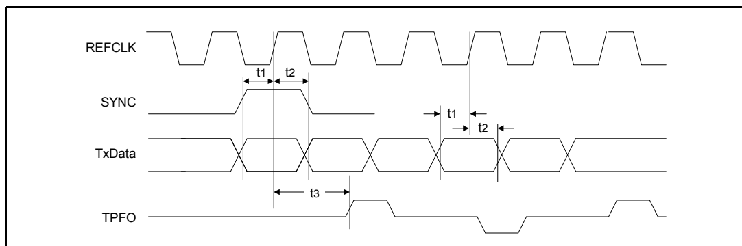
Figure 42 SMII - 100BASE-FX Transmit Timing
