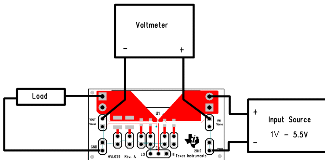
Figure 1. R_{ON} Setup
