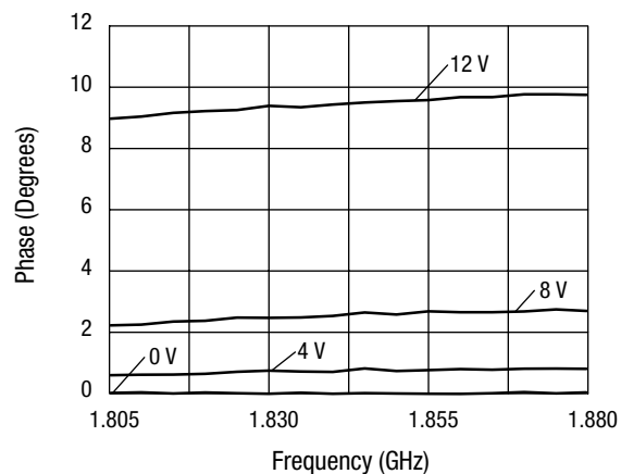
Phase vs. Frequency and Control Voltage — DCS Band
