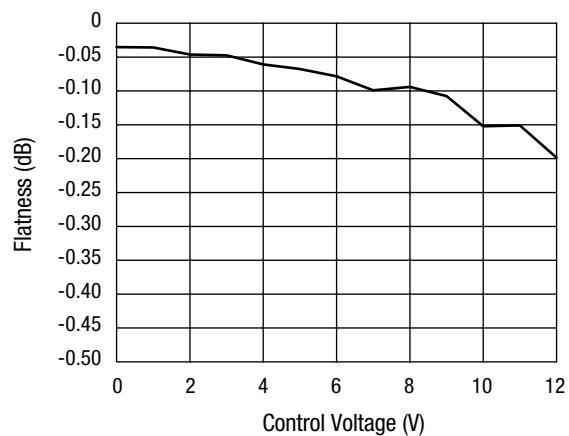
Insertion Loss Flatness vs. Control Voltage — DCS Band
