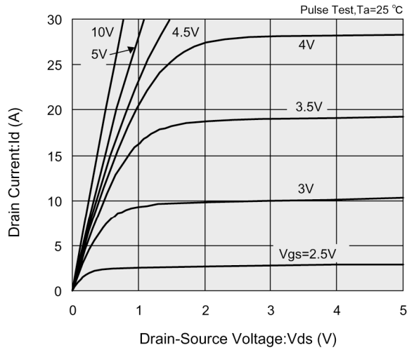
(1) Drain Current vs. Drain-Source Voltage
