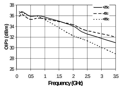
OIP_3 vs. Frequency
