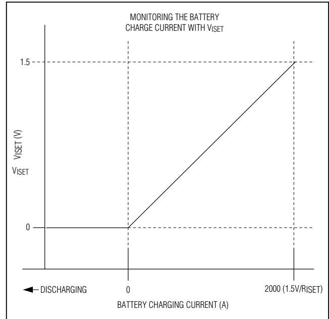
Figure 4. Monitoring the Battery Charge Current with \text{V}_{\text{ISET}}
