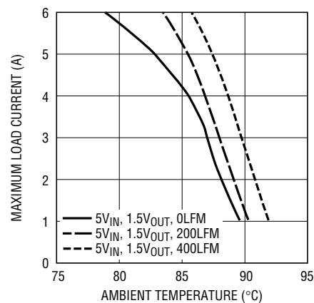
Figure 9. No Heat Sink
