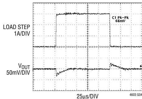
1.2V Transient Response
