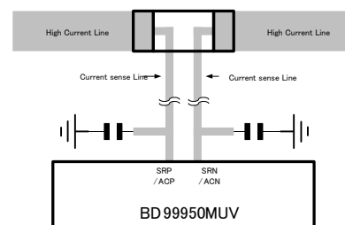
Figure 25. Current Sense Kelvin Layout
