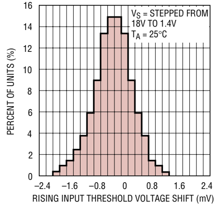
Distribution of Power Supply Rejection
