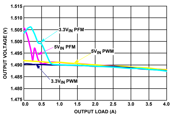
FIGURE 9. V_{OUT} REGULATION vs LOAD (1MHz, V_{OUT} = 1.5\text{V} )
