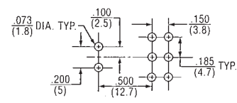
2 Pole P.C. Mounting
