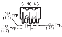
1 Pole P.C. Mounting
