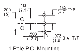
1 Pole P.C. Mounting
