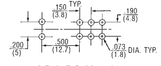
2 Pole P.C. Mounting
