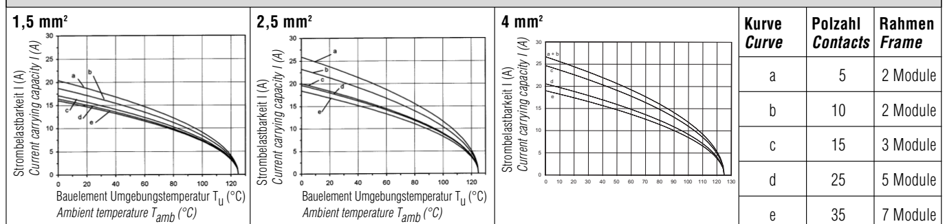
Derating Kurven / Derating curves
