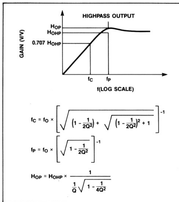
Figure 4. Highpass Response
