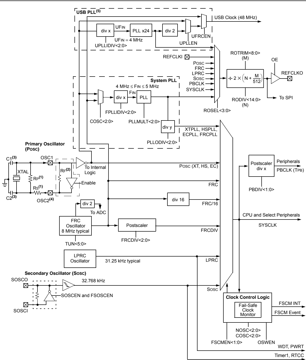
FIGURE 8-1: OSCILLATOR DIAGRAM
