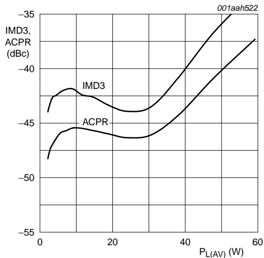
Fig 7. Adjacent channel power ratio and third order intermodulation distortion as function of average output power; typical values
