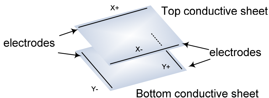
Figure 10 – 4-wire Touchscreen
