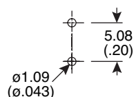
P.C. MOUNTING
