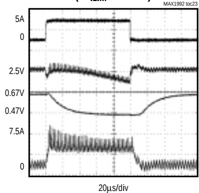
INDUCTOR SATURATION PROTECTION ( \Delta V_{ILIM} = 200mV )
