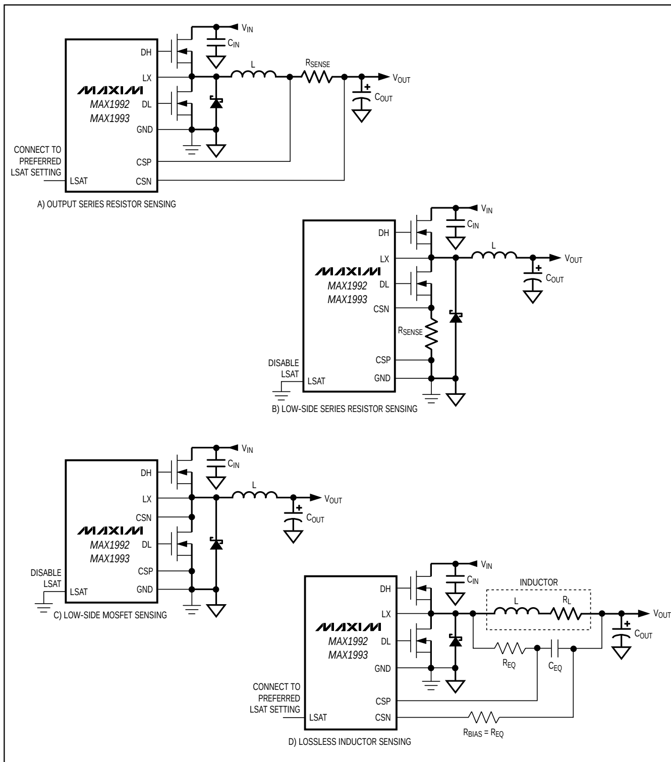
Figure 10. Current-Sense Configurations
