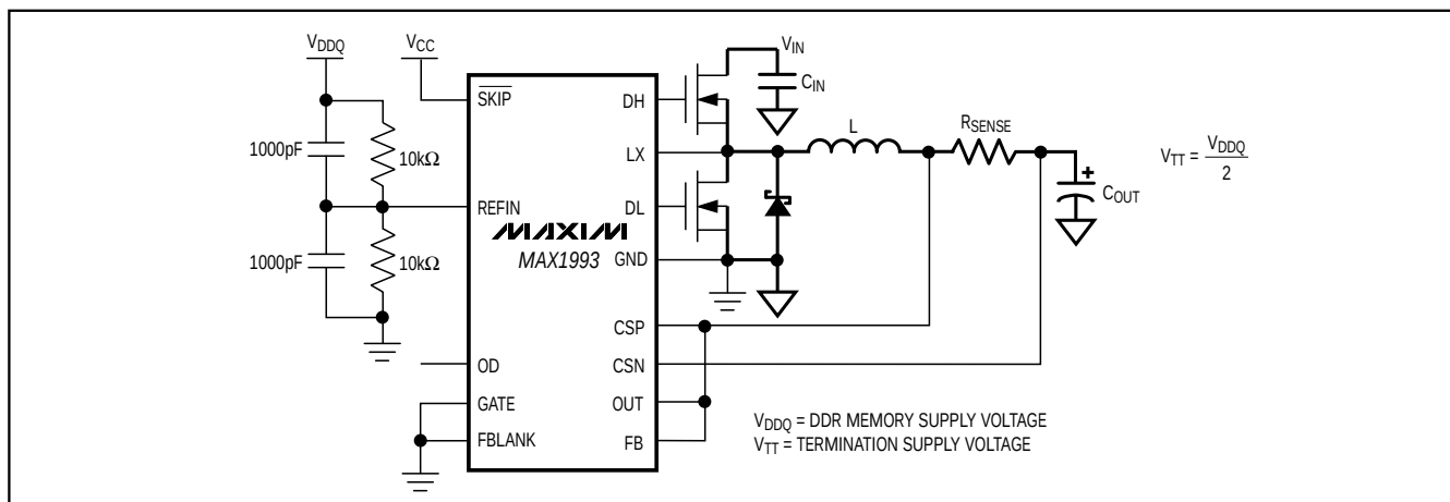
Figure 12. Active Bus Termination
