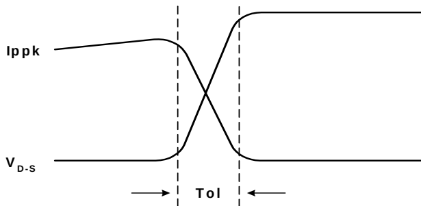
FIGURE 6. SWITCHING CYCLE
