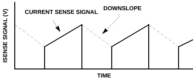
FIGURE 5. SLOPE COMPENSATION
