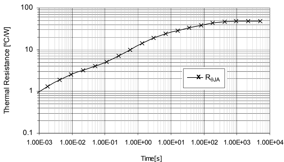
Figure 28. Transient Pin Resistance R_{\theta JA} Device on Thermal Test Board Area A = 600 (mm²)
