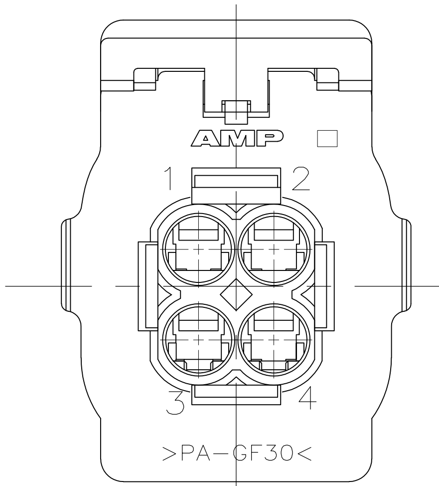
VIEW B-B
