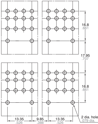
Side-by-side installation
