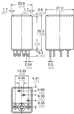
External dimensions
