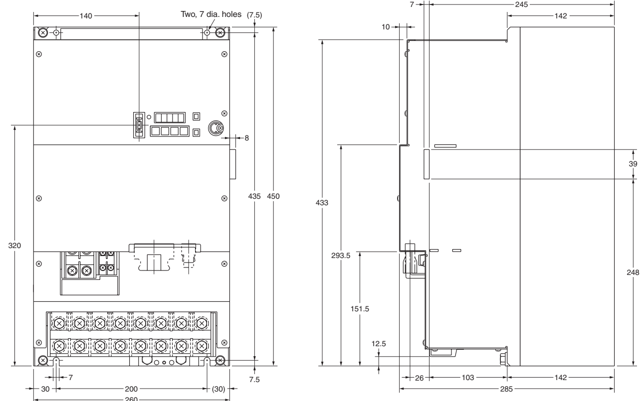
Mounting hole dimensions
