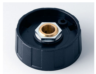
A2540080 ROUND KNOB 40, without line ABS (UL 94 HB) black RAL 9005 40x15mm 8mm
