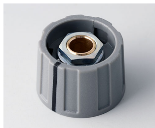
A2623068 ROUND KNOB 23, with line ABS (UL 94 HB) dusty gray RAL 7037 23x15mm 6mm
