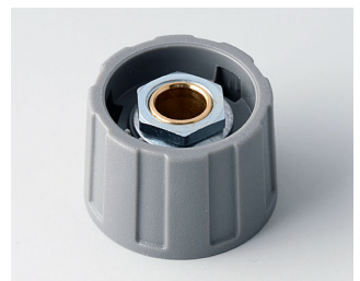
A2523068 ROUND KNOB 23, without line ABS (UL 94 HB) dusty gray RAL 7037 23x15mm 6mm
