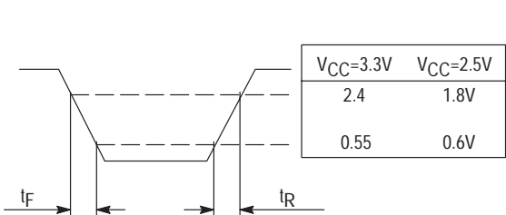
Figure 7. Output Transition Time Test Reference
